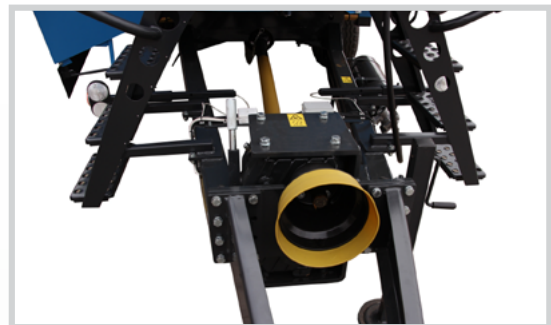
Two-gear transmission
